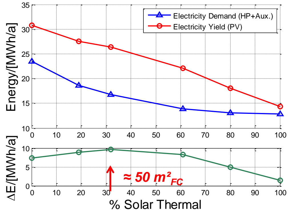
Electricity Demand and PV yield
